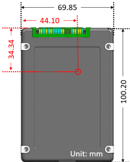
[Figure 2] Thermal Probe Location (15.36TB~ 30.72TB)
