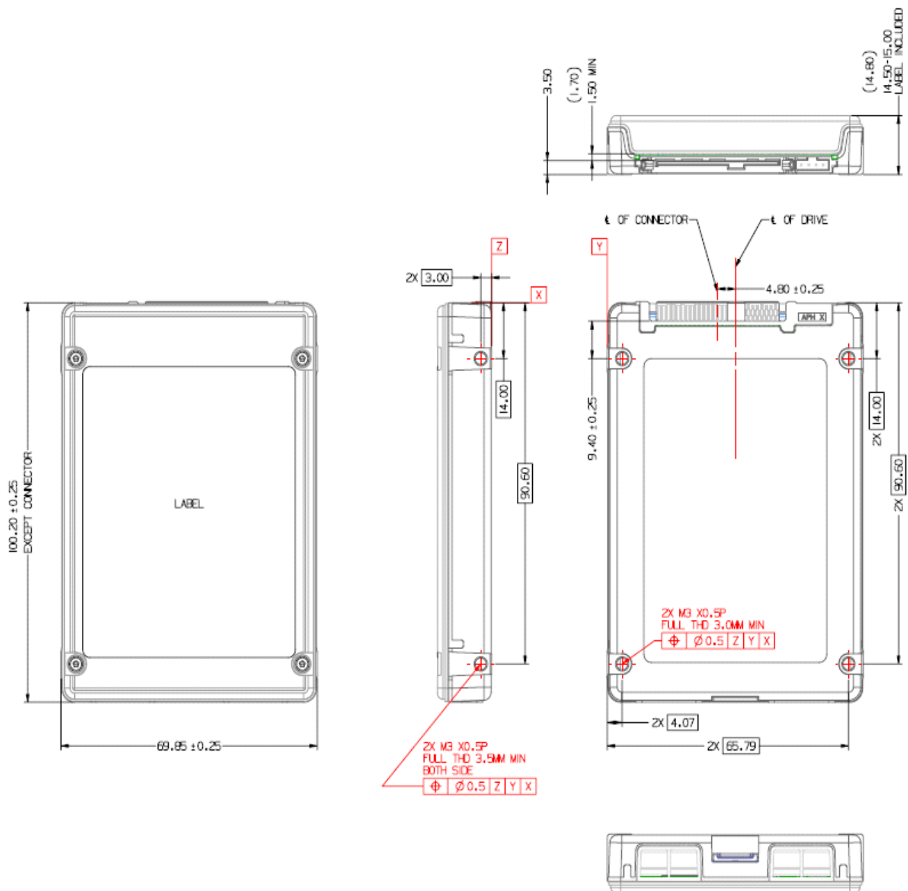
[Figure 3] Mechanical Outline
