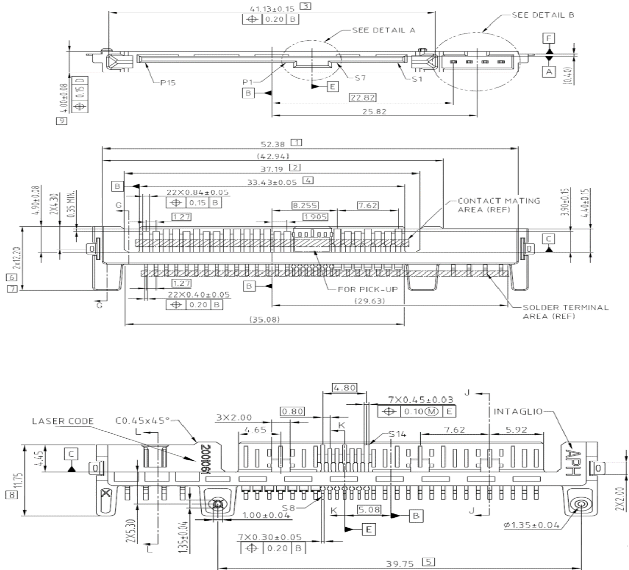
[Figure 4] Layout of 2.5-inch Form Factor Connector Pins
