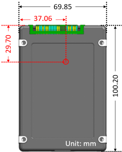
[Figure 1] Thermal Probe Location (960GB~7.68TB)
