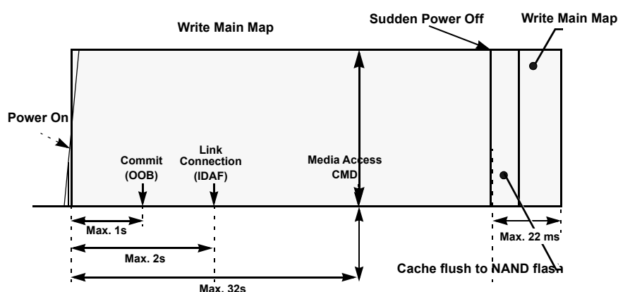
[Figure 5] Time to Ready Sequence
